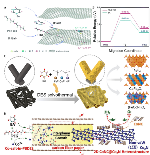
Fig. 3 Fabrication of self-supporting electrodes. (A) Schematic illustrating the migration path of BA and PEG 200 entering the graphitic layers and the corresponding binding energy. (B) Migration energy diagram of BA and PEG 200 entering the graphitic layers. Reprinted with permission from copyright© Royal Society of Chemistry, 2021. 39 (C) Schematic illustration of the universal preparation of 2D spinel oxides. Reprinted with permission from copyright© Elsevier Ltd, 2022. 41 (D) Schematic illustration of the fabrication process of 2D \text{CoNC}@\text{Co}_2\text{N} heterostructures for water splitting. Reprinted with permission from copyright© Wiley-VCH GmbH, 2020. 43
