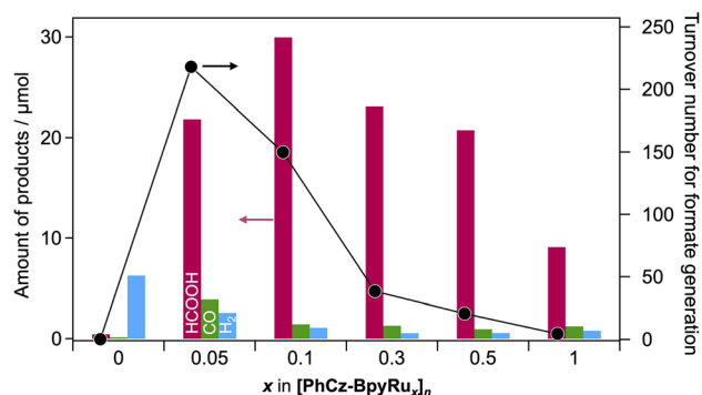
Fig. 5 Amounts of formate, CO, and H 2 formation generated over [PhCz-BpyRu] x (2 mg) with different loading amounts of Ru complex moiety ( x = 0, 0.05, 0.1, 0.3, 0.5 , and 1) in MeCN–TEOA (4 : 1, v/v, 2 mL) under irradiation of \lambda > 380 nm light for 6 h.
