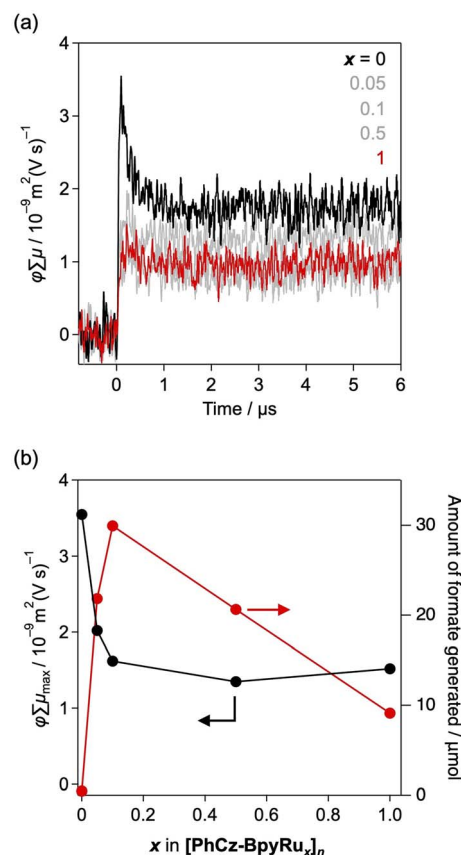
Fig. 6 (a) Transient photoconductivities upon laser pulse excitation at 355 nm of [PhCz-BpyRu] x with different loading amounts of Ru complex moiety. (b) Dependence of maximum transient conductivities \phi\Sigma\mu_{\max} and amounts of formate production on the amount of Ru complex hybridised.
