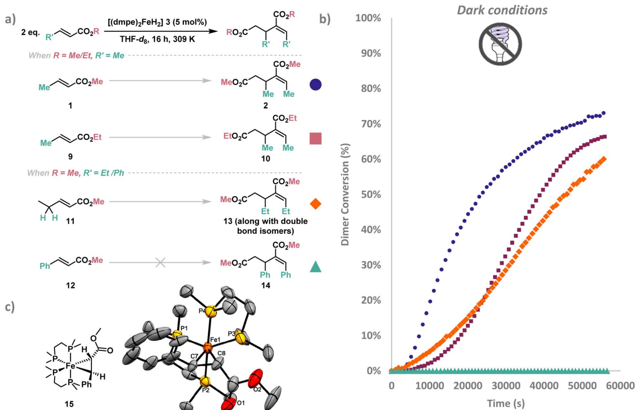
Fig. 1 (a) in situ Monitoring of crotyl substrates 1 , 9 , 11 and 12 under dark conditions with [(\text{dmpe})_2\text{FeH}_2] 3 (5 mol%) in \text{THF-d}_8 at 309 K were converted to dimers 2 , 10 , 13 and 14 respectively. The substrates selected either had a different alkyl ester ( R = \text{Me}, \text{Et} ) or different substituents at the vinylogous position ( R' = \text{Me}, \text{Et}, \text{Ph} ). Product 13 was formed along with double bond isomers as the major products (see SI S9 SI Fig. 45–47 for additional details). (b) The dimer conversion (%) over time (s) across 16 hours under dark conditions. Dimer conversion (%) was calculated by integrating ^1\text{H} resonances corresponding to starting material and dimer products, then computing (dimers/(dimers + starting material)) \times 100%. (c) ORTEP plot of [\text{Fe}(\text{PhCH}=\text{CHCO}_2\text{Me})(\text{dmpe})_2] 15 , hydrogens have been omitted for clarity and X-ray ellipsoids have been set at 50% probability.
