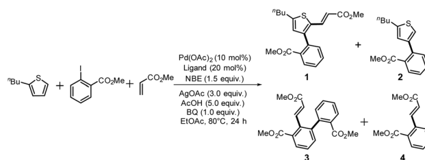
Scheme 1 Catalytic C–H difunctionalization reaction of thiophene, yielding the difunctionalized product 1 , monofunctionalized product 2 , Catellani product 3 , and Heck product 4 .
