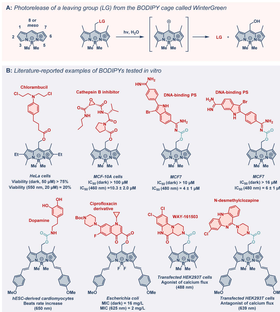
Fig. 1 (A) Photorelease of a leaving group (LG) from the BODIPY cage called WinterGreen. (B) Known examples of photocaged compounds for biological applications. \text{IC}_{50} is a half-maximal inhibitory concentration, MIC is a minimum inhibitory concentration with indicated irradiation wavelength and without irradiation (dark). The cell lines or bacteria used are indicated in italics. 11,13,21,29
