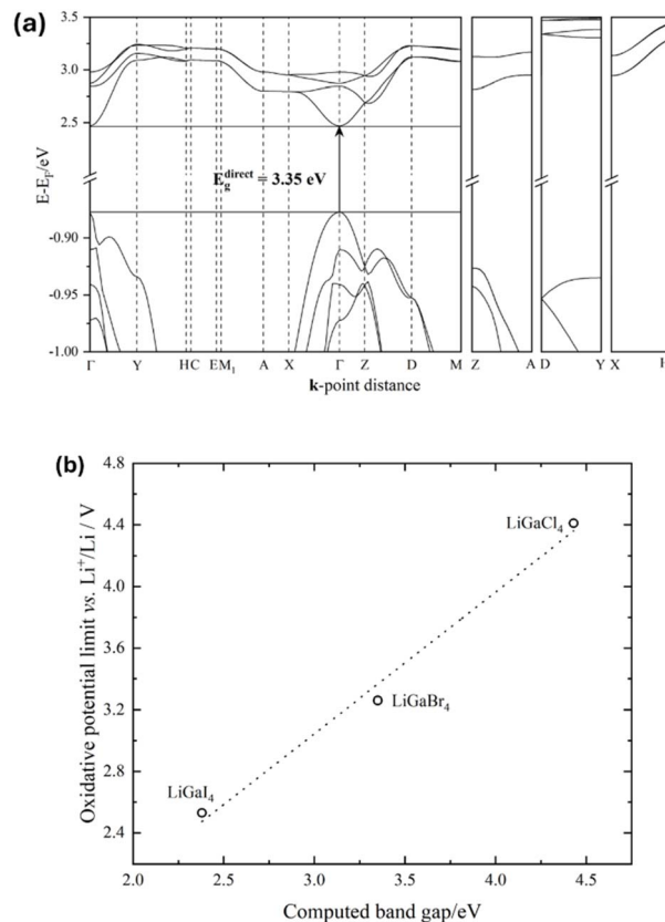
Fig. 3 (a) Computed (DFT/PBE) band structure of LiGaBr 4 with band energies scaled to the Fermi level ( E_F ). (b) Correlation between computed oxidative potential 12 and computed band gap energies of LiGaX 4 (X = Cl, Br, I) materials. The dotted line corresponds to a linear fit ( R^2 = 0.991 ).
