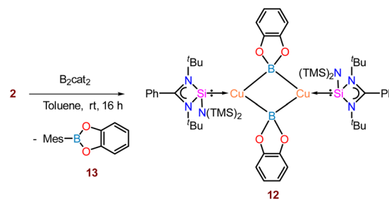
Scheme 3 Reaction of complex 2 with a diboron compound (B 2 cat 2 ).
