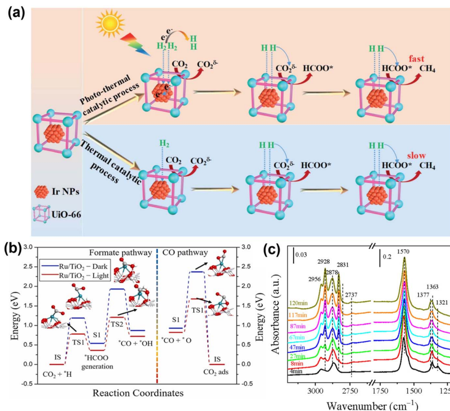
Fig. 13 (a) Proposed reaction mechanism for the thermal and photo-thermal catalytic Sabatier reaction over Ir@UiO-66. 118 Copyright 2022, Royal Society of Chemistry. (b) Feasible routes of the \text{CO}_2 hydrogenation reaction on the Ru/TiO 2 model surface under dark and light conditions. 119 Copyright 2022, Elsevier. (c) In situ DRIFT spectra obtained from the surface species formed during the reaction for 3.5% Cd/TiO 2 . 120 Copyright 2022, Elsevier.
