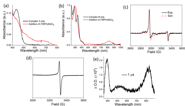
Fig. 8 UV-visible absorption spectra of (a) complex 1 and (b) complex 5 before and after the addition of 1 equiv. (TBPA)SbCl 6 in a mixed CH 2 Cl 2 /MeCN solution (2 : 1 v/v) at -40^\circ\text{C} . (c) X-band EPR spectrum (solid, black) of the reaction mixture of 1 (3 mM) and 0.5 equiv. (TBPA)SbCl 6 in frozen CH 2 Cl 2 at 100 K; spectral simulation (dash, red) revealed that the spectrum comprises 75% Pd II –Pd III species ( 1 + ) and 25% organic radicals. (d) X-band EPR spectrum of the reaction mixture of 5 (3 mM) and 0.5 equiv. (TBPA)SbCl 6 in frozen CH 2 Cl 2 at 100 K. (e) ns-TA spectrum recorded at 1 \mu\text{s} after flashing a deoxygenated MeCN/toluene (1:9 v/v) solution of complex 5 ( 2 \times 10^5 \text{ s}^{-1} ) and 4-(methoxycarbonyl)- N -methylpyridinium hexafluorophosphate (0.001 M) at RT.
