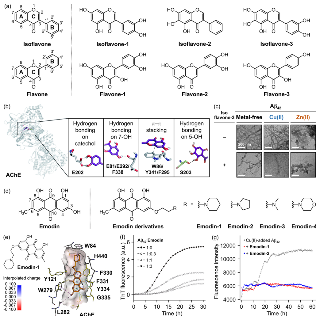
Fig. 8 Examples of chemical reagents regulating metal-free or metal-bound Aβ and AChE. (a) Structures of flavonoids. Isoflavone , 3-phenyl-4 H -chromen-4-one; isoflavone-1 , 3-(3,4-dihydroxyphenyl)-5,7-dihydroxy-4 H -chromen-4-one; isoflavone-2 , 5,6,7-trihydroxy-3-phenyl-4 H -chromen-4-one; isoflavone-3 , 3-(3,4-dihydroxyphenyl)-5,6,7-trihydroxy-4 H -chromen-4-one; flavone , 2-phenyl-4 H -chromen-4-one; flavone-1 , 2-(3,4-dihydroxyphenyl)-3,5,7-trihydroxy-4 H -chromen-4-one; flavone-2 , 2-(3,4-dihydroxyphenyl)-5,7-dihydroxy-4 H -chromen-4-one; flavone-3 , 2-(4-hydroxyphenyl)-3,5,7-trihydroxy-4 H -chromen-4-one. (b) Intermolecular interactions between the flavonoids and AChE. Reproduced with permission from ref. 289 and 292. Copyright© 2023 Royal Society of Chemistry and 2020 Royal Society of Chemistry. (c) Impact of isoflavone-3 on the formation of metal-free Aβ 42 and metal-Aβ 42 aggregates. The morphology of the resultant Aβ 42 species was analyzed by TEM. Reproduced with permission from ref. 289. Copyright© 2023 Royal Society of Chemistry. (d) Structures of emodin and its derivatives with different functional groups at the R position. Emodin , 1,3,8-trihydroxy-6-methylanthracene-9,10-dione; emodin-1 , 1,8-dihydroxy-3-methyl-6-(2-(piperidin-1-yl)ethoxy)anthracene-9,10-dione; emodin-2 , 1,8-dihydroxy-3-methyl-6-(2-(pyrrolidin-1-yl)ethoxy)anthracene-9,10-dione; emodin-3 , 1,8-dihydroxy-3-methyl-6-(2-(dimethylamino)ethoxy)anthracene-9,10-dione; emodin-4 , 1,8-dihydroxy-3-methyl-6-(2-morpholinoethoxy)anthracene-9,10-dione. (e) Binding of emodin-1 against AChE. Reproduced with permission from ref. 291. Copyright© 2024 Elsevier. (f) Effect of emodin on Aβ 42 aggregation. The inhibitory activity of emodin on the production of β-sheet-rich Aβ 42 aggregates was quantitatively measured by the ThT assay. Reproduced with permission from ref. 101. Copyright© 2021 John Wiley and Sons. (g) Impact of emodin-1 and emodin-2 on Cu(II)-induced Aβ 42 aggregation. The influence of emodin-1 and emodin-2 on the generation of β-sheet-rich Cu(II)-Aβ 42 aggregates was analyzed by the ThT assay. Reproduced with permission from ref. 293. Copyright© 2023 Springer Nature.
