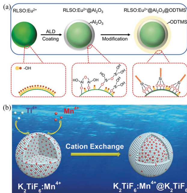
Fig. 7 (a) Schematic illustration of surface coating via atomic layer deposition (ALD) for the RLSO: \text{Eu}^{2+} phosphor and subsequent hydrophobic surface modification with ODTMS on RLSO: \text{Eu}^{2+} @ \text{Al}_2\text{O}_3 surface. Reproduced with permission from ref. 166. Copyright 2020, WILEY-VCH. (b) Illustration of the construction of KTF: \text{Mn}^{4+} @KTF core-shell phosphor through a reverse cation-exchange strategy. Reproduced with permission from ref. 161. Copyright 2019, WILEY-VCH.
