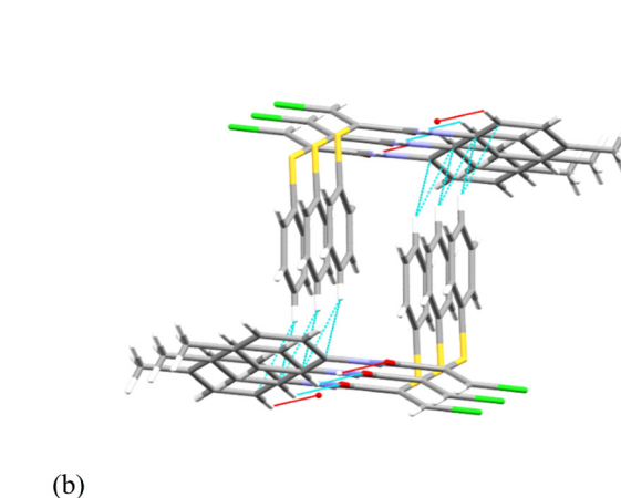
Fig. 5 Views, (a) and (b), from different angles showing the knitting of two chains of Z-3 together based on edge-to-face ( C-H\cdots\pi 2.83 Å) and face-to-face aromatic interactions.
