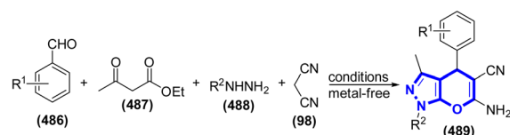
Scheme 130 Synthesis of pyrano[2,3-c]pyrazoles catalyzed by metal-free catalysts.
