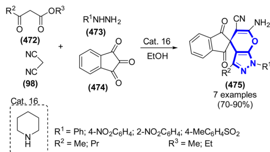
Scheme 127 Synthesis of spiro-pyrano[2,3-c]pyrazoles and oxa-aza-[3.3.3]propellanes catalyzed by Cat. 16 in ethanol.
