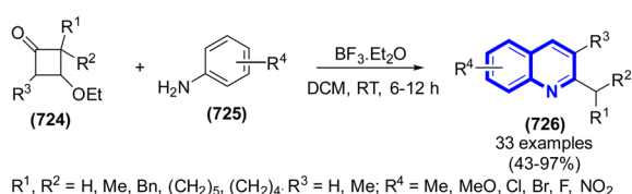
Scheme 204 Synthesis of quinolones catalyzed by \text{BF}_3 \cdot \text{OEt}_2 .
