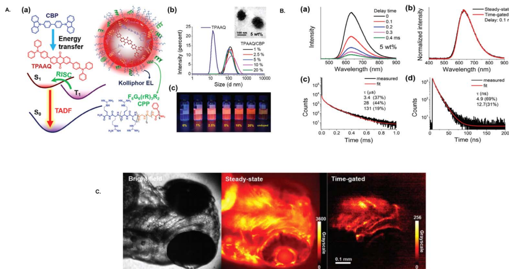
Fig. 24 (A) (a) Representation of TPAAQ/CBP/CPD TADF nanoparticles (b) DLS histograms showing the size of the nanoparticles and inset TEM images showing their morphology. (c) Photographs of the nanoparticle solutions under UV irradiation. (B) Time-gated emission spectra of the nanoparticles at various delay times. (C) Imaging of zebrafish incubated with TPAAQ/CBP/CPD nanoparticles, where the bright field is displayed on the left side of the figure, the steady-state luminescence is shown in the middle, and the time-gated luminescence is displayed on the right. Reproduced from ref. 173 with permission from John Wiley & Sons, Copyright © 2024, Wiley-VCH Verlag GmbH & Co. KGaA, Weinheim.
