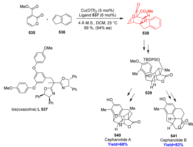
Scheme 70 IEDDA reaction of 2-pyrone 535 with indane 536 in the total synthesis of cephanelide A ( 540 ), and cephanelide B ( 541 ). 140
