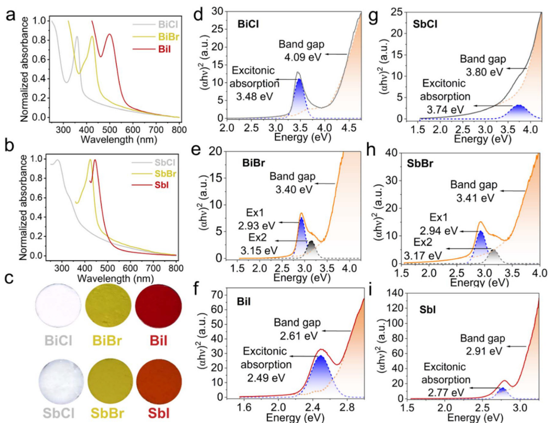
Fig. 6 (a and b) Normalized UV-vis absorbance spectra; (c) photographs of perovskite powder ( (\text{AzrH})_3\text{M}_2\text{Cl}_9 – white, (\text{AzrH})_3\text{M}_2\text{Br}_9 – yellow, and (\text{AzrH})_3\text{M}_2\text{I}_9 – red); (d–i) Tauc plots for direct band gap semiconductors. The direct bandgap semiconducting nature of the reported perovskites was confirmed by DFT calculations as shown further in the text.
