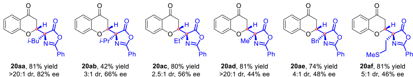
Fig. 5 Selected examples from the general scope of the decarboxylative Michael addition of azlactones 18a–f to chromone-3-carboxylic acid 17a .
