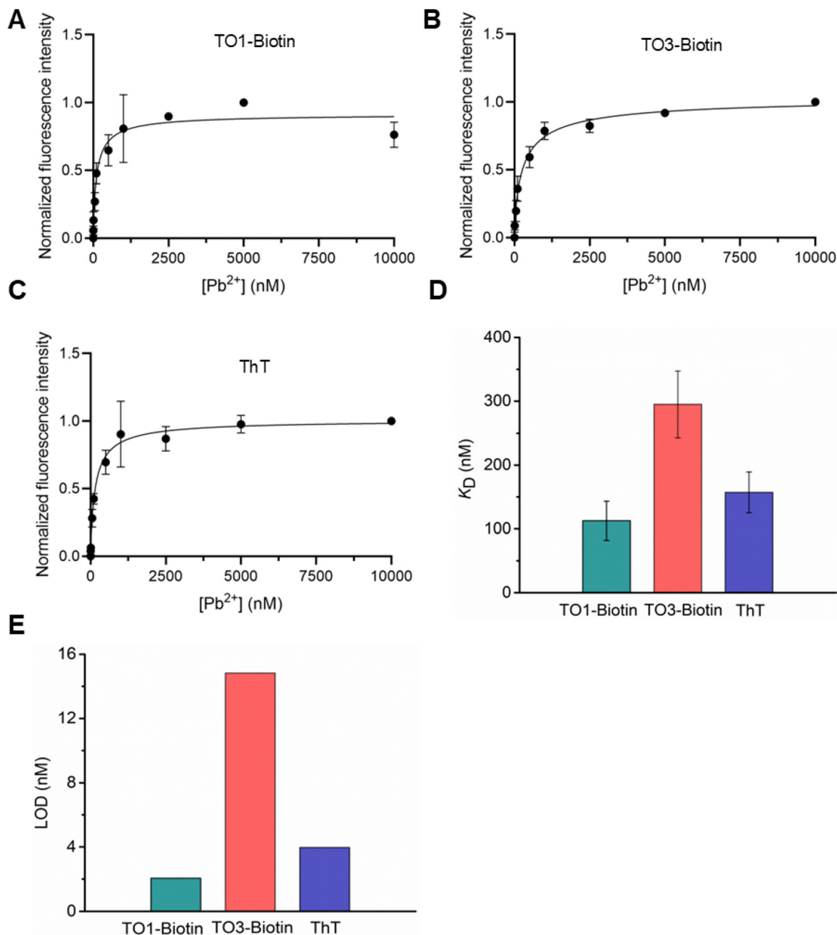
Fig. 4 RNA Mango exhibits high sensitivity for Pb^{2+} detection. (A–C) Fluorescence signals exhibited by RNA Mango in response to increasing concentrations of Pb^{2+} with (A) TO1-biotin, (B) TO3-biotin, and (C) ThT. (D) RNA Mango binds to Pb^{2+} with high affinity in the presence of all three dyes, exhibiting K_D values of 100–300 nM. (E) RNA Mango is highly sensitive to low nanomolar concentrations of Pb^{2+} in the presence of all three dyes, with LOD of 2–16 nM. Experiments were performed at pH 8 and 5 mM Mg^{2+} . Concentrations of RNA and the dye were 100 nM and 1 \mu M, respectively, with Pb^{2+} concentrations in the range of 5 nM–10 \mu M. Error bars correspond to the standard deviation of three independent experiments.
