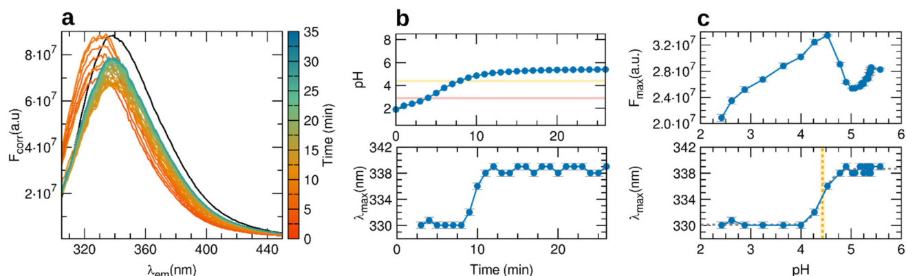
Fig. 3 (a) Fluorescence spectra of HSA (0.055 mM) after the addition of 20 mM 1 as a function of time, as indicated by the colour bar ( T = 25^\circ\text{C} ). The emission spectrum of the initial stock solution is reported as a black line. (b) Plot of the measured pH value (top panel) and the position of the fluorescence emission maximum ( \lambda_{\text{max}} , lower panel) as a function of time. (c) Plot of the maximum fluorescence intensity ( F_{\text{max}} ) and of \lambda_{\text{max}} as a function of pH, according to a concomitant pH–time calibration. The \lambda_{\text{max}} vs. pH profile was fitted using a sigmoid function
