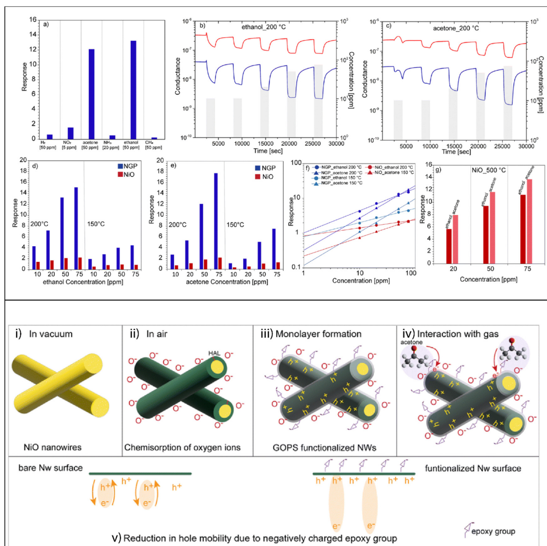
Fig. 19 (a) Response of the NGP sensor toward different gas analytes. (b and c) Dynamic response of NiO (red) and NGP (blue) sensors toward the different concentrations of ethanol and acetone (10, 20, 50, and 75 ppm) in dry air at 200 °C. (d and e) Response vs. concentration curves of bare NiO and NGP at 200 °C and 150 °C toward ethanol and acetone. (f) Calibration curves of the NiO and NGP sensors for ethanol and acetone. (g) Response vs. concentration graph of the NiO sensor toward ethanol and acetone at 500 °C. (i) NiO nanowires in a vacuum. (ii) Chemisorption of oxygen ions ( O^{2-} ) occurs on the surface of NiO NWs, which leads to the formation of a narrow hole accumulation layer (HAL) around the resistive core. (iii) Monolayer formation on the NWs surface that leads to the accumulation of holes near the surface due to the presence of negatively charged epoxy groups of GOPs. (iv) Enhanced interaction with acetone gas leads to an increase in electron–hole recombination as compared to bare NiO NWs. (v) Reduction in the hole mobility occurs after the functionalization with GOPs. Reproduced from ref. 50 with permission from RSC, copyright 2023.
