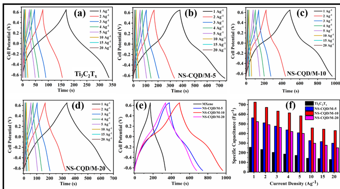
Fig. 7 GCD curves of (a) \text{Ti}_3\text{C}_2\text{T}_x , (b) NS-CQD/M-5, (c) NS-CQD/M-10, (d) NS-CQD/M-20, (e) all the composites in comparison with pristine \text{Ti}_3\text{C}_2\text{T}_x at a fixed current density of 1 \text{A g}^{-1} , and (f) comparison of specific capacitances of all the composites at varying current densities.
