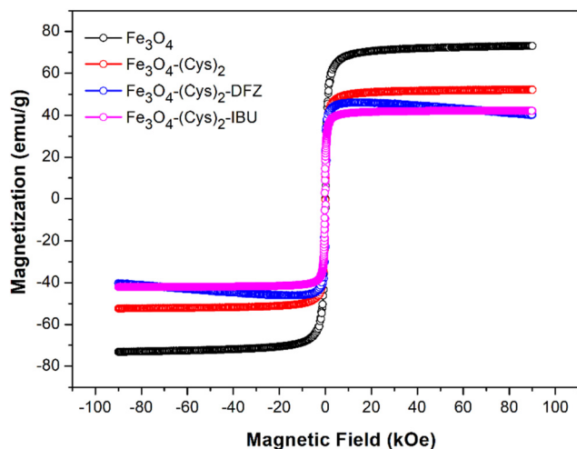
Fig. 10 Magnetization curves of (a) \text{Fe}_3\text{O}_4 (black line), \text{Fe}_3\text{O}_4 -(Cys) 2 (red line) and \text{Fe}_3\text{O}_4 -(Cys) 2 -DFZ (blue line) (b) \text{Fe}_3\text{O}_4 -(Cys) 2 -IBU (magenta line).
