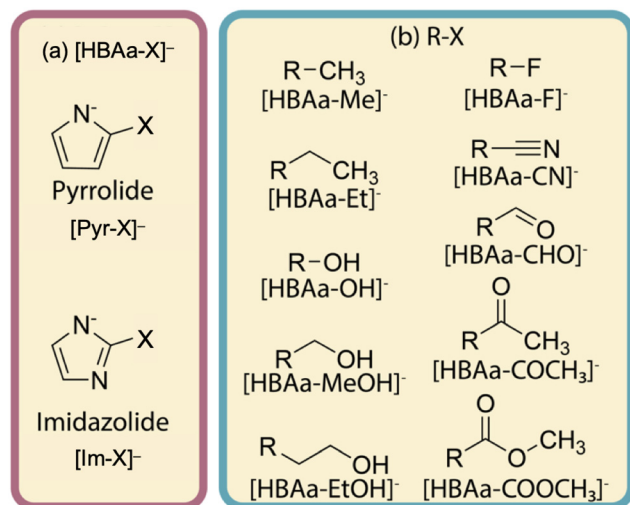
Fig. 2 [\text{Pyr-X}]^- and [\text{Im-X}]^- (a) were investigated for the influence of functionalization with the ten different functional groups (X) shown in (b). In part (b), electron-donating groups are shown in the left column while electron-withdrawing groups are shown in the right column.
