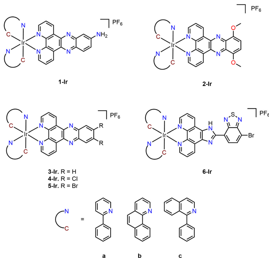
Fig. 28 Structures of C^N cyclometalated Ir(III) compounds (1a-Ir–6c-Ir).
