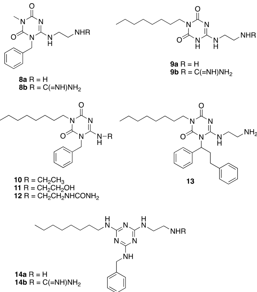
Fig. 3 Analogues lacking key functional groups or additional groups.
