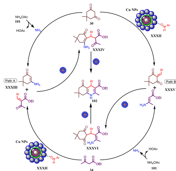
Fig. 11 Plausible mechanism for synthesis of hexahydroquinoline derivatives using an Fe 3 O 4 @SiO 2 @Si-(CH 2 ) 2 @HMTA@Cu nanocomposite (Salem et al. ).
