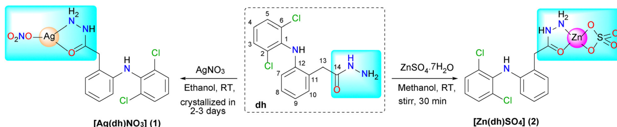
Scheme 1 Synthetic pathway for metal complexes of dh : 1 ( \text{Ag}^{\text{I}} ) and 2 ( \text{Zn}^{\text{II}} ).
