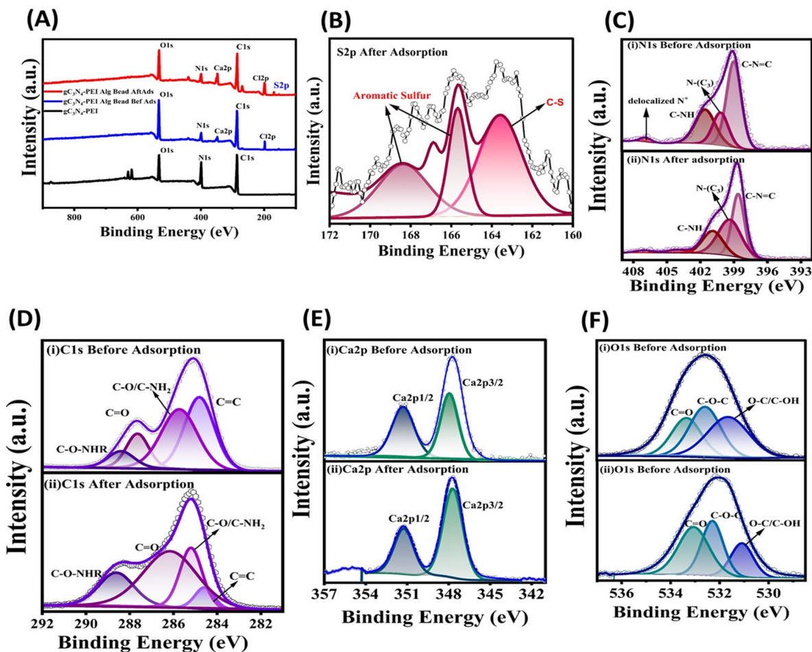
Fig. 1 (A) The total survey spectra of PEI exfoliated g\text{-C}_3\text{N}_4 NSs, and also PEI exfoliated g\text{-C}_3\text{N}_4\text{NSs@Cal-Alg} beads before and after adsorption of DBT; (B)–(F) high-resolution deconvoluted spectra before and after adsorption of the DBT spectra for sulphur (B), nitrogen (N 1S) (C), carbon spectra C 1S (D), calcium (Ca 2p) spectra (E), and oxygen (O 1S) spectra (F).
