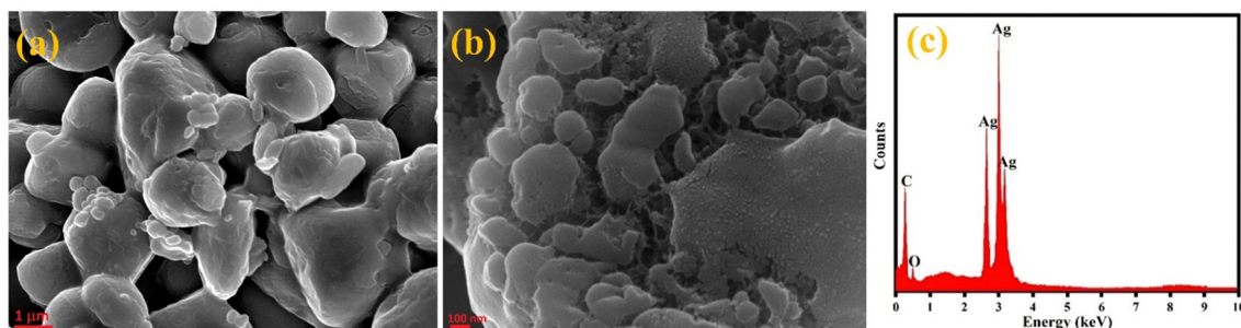
Fig. 4 SEM micrographs at (a) 1 \mu m (b) 100 nm and (c) EDX spectrum of TGRAgNPs .
