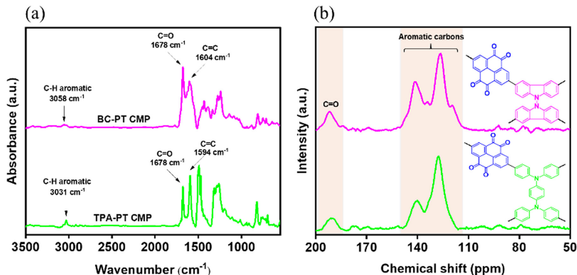
Fig. 1 (a) FTIR, and (b) solid-state 13 C CP/MAS NMR spectra of BC-PT, and TPA-PT CMPs.
