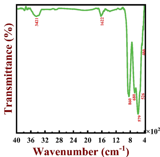
Fig. 4 FTIR spectrum of \text{CoWO}_4 nanostructures.
