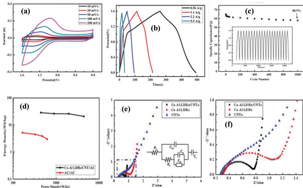
Fig. 14 (a) CV of asymmetric SC (CoAl LDH-CNT//AC). (b) GCD curve of CoAl LDH-CNT//AC. (c) Cycling stability. (d) Ragone plot of energy density vs. power density. (e) EIS spectra of CNTs, LDH, and LDH/CNT. (f) Magnified view of EIS. Reproduced with permission from ref. 73.
