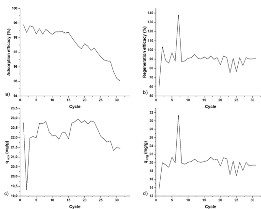
Fig. 11 Adsorption efficacy (%) (a), regeneration efficacy (%) (b), q_{\text{ads}} (mg g -1 ) (c), and q_{\text{reg}} (mg g -1 ) (d) for 31 consecutive adsorption–regeneration cycles of Cu.
