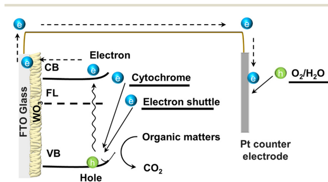
Fig. 5 Schematic diagram of the photocurrent generation by the WO 3 electrode with MR-1 bacteria. FL, CB, and VB represent the fermi level, conduction, and valence bands, respectively.
