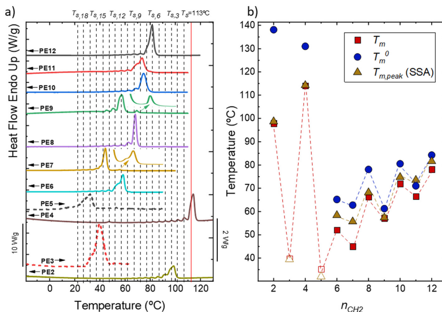
Fig. 13 (a) Final heating after the SSA protocol was applied to the indicated samples. We used the following conditions for the SSA protocol: T_{s,\text{ideal}} = 113 °C, a fractionation window of 5 °C, and scan rates of 20 °C \text{min}^{-1} . (b) T_m , T_m^0 and T_{m,\text{peak}}(\text{SSA}) as a function of n_{\text{CH}_2} .
