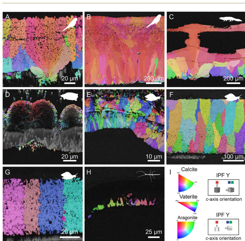
Fig. 3 EBSD maps of radially sectioned eggshells. Inverse pole figure (IPF) maps displaying the crystalline structure, and orientation of the calcium carbonate crystals in the shells. (A) Psittacula roseata (Aves), (B) Rhea americana (Aves), (C) Caiman crocodilus (Reptilia). Except for the turtle (D) Pelusios carinatus (Reptilia) that presents the aragonite polymorph, all other vertebrates show calcite crystals. In invertebrates, (E) shows a rare occurrence of vaterite in the eggshell of Pomacea canaliculata (Gastropoda) while the other snails (F) Archachatina marginata (Gastropoda) and (G) Achatina fulica (Gastropoda) have calcite. (H) Clear calcite crystals were also visible in the stick insect Heteropteryx dilatata (Insecta). (I) Legends for inverse pole figure Y maps and a schematic representation of c-axis orientation for calcium carbonate polymorphisms: calcite and vaterite for which the crystals are hexagonal and aragonite with an orthorhombic shape.
