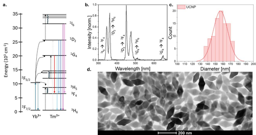
Fig. 2 (a) Energy-level diagram illustrating the upconversion mechanism facilitated by Yb 3+ and Tm 3+ ions in the UCNP. The UCNP are composed of LiYF 4 doped with 0.5 mol% Tm 3+ and 25 mol% Yb 3+ . (b) Emission spectrum of the UCNP, showing efficient generation of UV light upon excitation at 980 nm. (c) Size distribution of the synthesized UCNP, revealing a particle diameter of 135–175 nm. (d) Transmission electron microscopy (TEM) image of diamond-shaped UCNP. 29,30
