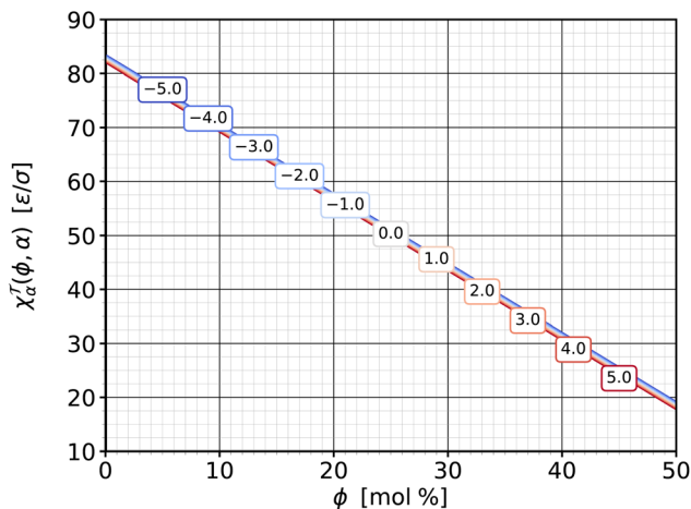
Fig. 9 Susceptibility \chi_{\alpha|\phi}^T from eqn (13b) as a function of cholesterol content \phi , parametrized by different values of phospholipid abundance \alpha , as indicated in the boxed labels. The lines almost coincide, with smaller \alpha values having ever so slightly larger susceptibilities.
