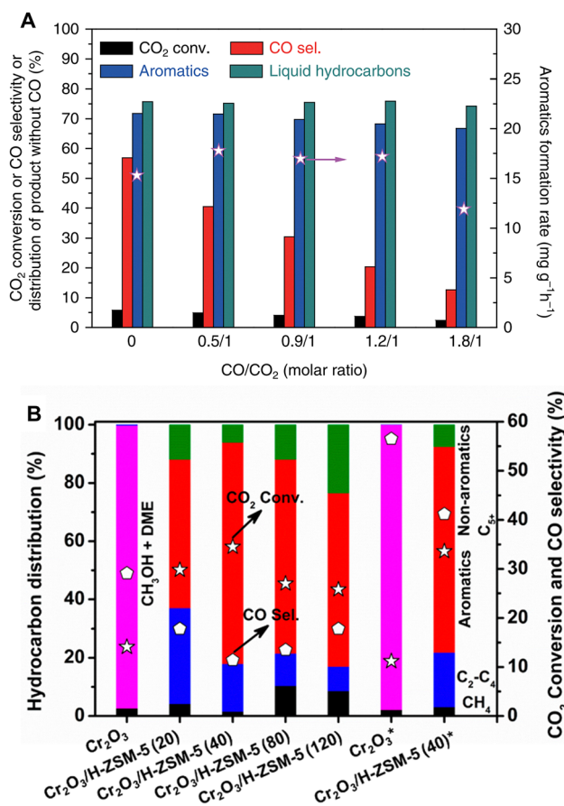
Fig. 17 The coupling of CO_2 hydrogenation with CO hydrogenation. (A) 667 mg of ZnAlO_x /H-ZSM-5, 320 °C, 3.0 MPa, H_2/CO_2/Ar = 3/1/0.2 , 66.7 mL min^{-1} , CO = 0-26.6 mL min^{-1} . Reprinted with permission from Ni et al. Copyright (2018), The Authors. 41 (B) 0.25 g of Cr_2O_3 or 0.5 g of Cr_2O_3 /H-ZSM-5, 350 °C, 3 MPa, H_2/CO_2 = 3 (5.42 vol% CO), 10 mL min^{-1} . * refers to the results without CO. Reprinted with permission from Wang et al. Copyright (2019), American Chemical Society. 55
