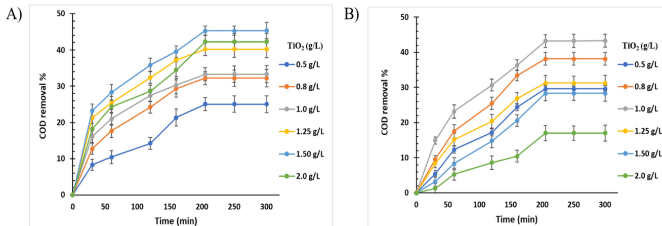
Fig. 8 Effect and COD removal vs. time: (A) for FULV and (B) for SUVL configurations.
