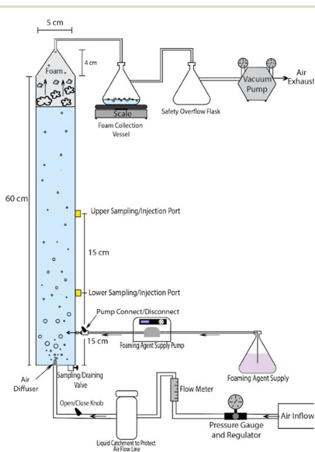
Fig. 1 Schematic diagram of the foam fractionation apparatus.
