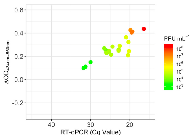
Fig. 3 Positive MS2 detections, by RT-qPCR cycle quantification (Cq) values plotted against the corresponding RT-LAMP \Delta\text{OD}_{434-560\text{nm}} measurements. Data points are colour-coded according to corresponding PFU \text{mL}^{-1} concentrations measured in parallel.
