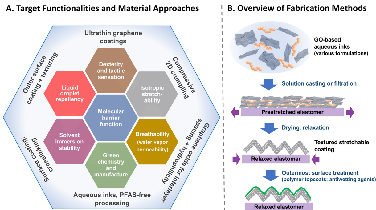
Fig. 1 Overall objectives and approach. A: Set of target properties for stretchable PPE coatings (hexagons), and the coating features and processing strategies used in the present study to address them (black text; outer rim). B: Overview of film fabrication steps and the corresponding material architectures.
