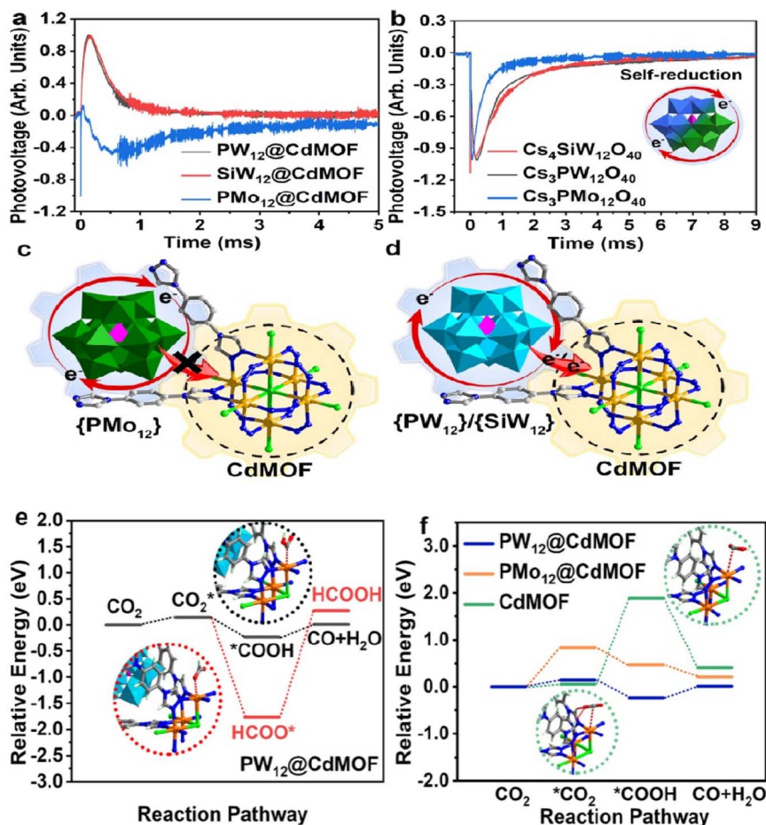
Fig. 7 (a) and (b) TPV curves of POM@CdMOF and cesium salt of parent POMs. (c) Graph of the \{PMo_{12}\} cluster in \text{PMo}_{12}@CdMOF . (d) Graph of the electron transfer pathway between the \{PW_{12}\}/\{SiW_{12}\} cluster and CdMOF. (e) Calculated relative energy diagrams for \text{CO}_2 reduction to \text{CO} or \text{HCOOH} . (f) DFT calculations of \text{CO}_2 reduction to \text{CO} were conducted on the optimized POM@CdMOF and CdMOF.
