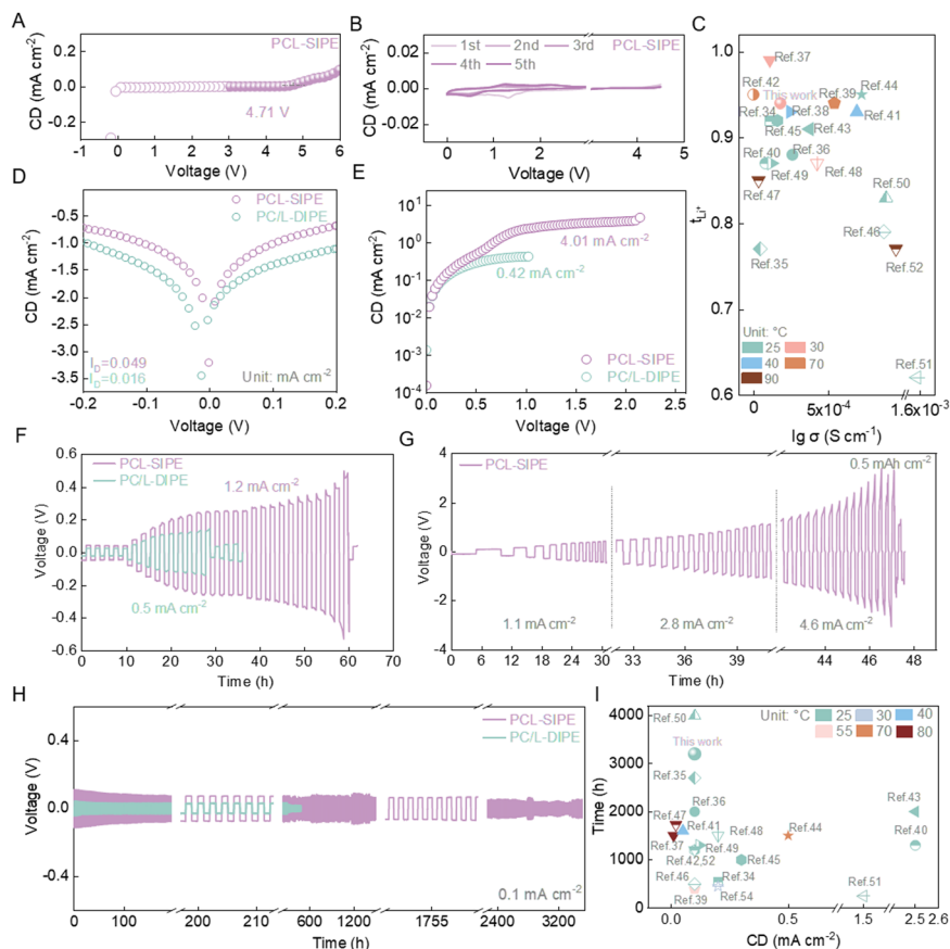
Fig. 3 Electrochemical performance of polymer electrolytes. (A) Electrochemical stability window of the PCL-SIPE (sweep rate: 0.2 \text{ mV s}^{-1} ). (B) Reduction (0.0–3.0 V) and oxidation (3.0–4.5 V) stability of the PCL-SIPE (Li|SS cells, sweep rate: 0.2 \text{ mV s}^{-1} ). (C) Comparison of t_{Li^+} and ionic conductivity with other reported SIPEs in the past three years. (D) Tafel curves of PCL-SIPE and PC/L-DIPE. (E) Limiting current density of PCL-SIPE and PC/L-DIPE. (F) CCD of the Li|PCL-SIPE|Li and Li|PC/L-DIPE|Li symmetric cells with a stripping-plating period of 1 h. (G) CCD of the Li|PCL-SIPE|Li symmetric cells with a fixed capacity of 0.5 \text{ mAh cm}^{-2} . (H) Cycling performance of the Li|PCL-SIPE|Li and Li|PC/L-DIPE|Li symmetric cells at a current density of 0.1 \text{ mA cm}^{-2} . (I) Comparison of the cycling performance with other reported SIPEs in the past three years.
