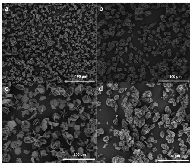
Fig. 11 FESEM images of EMM-17 obtained at \text{Ge}_f = 0.025 and water/ T = 10 with 7BMI (a) and 8BMI (b) at 7d and with 9BMI at 7d (c) and 12d (d).
