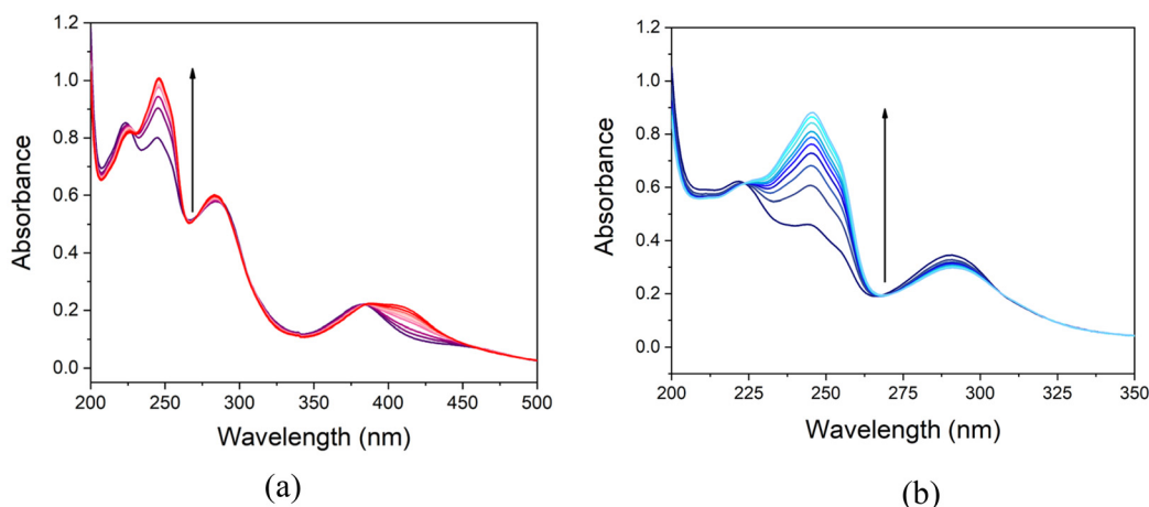
Fig. 3 Evolution of the electronic absorption spectra of the oxidation of H 2 Q into BQ ( \lambda_{\max} = 245 nm) catalysed by 1 (a) and 3 (b) at 25 °C under dioxygen saturation. The arrows indicate the course of the reaction during one hour. [\text{H}_2\text{Q}]_0 = 75 \mu\text{mol L}^{-1} and [\mathbf{1}] = [\mathbf{3}] = 7.5 \mu\text{mol L}^{-1} .
