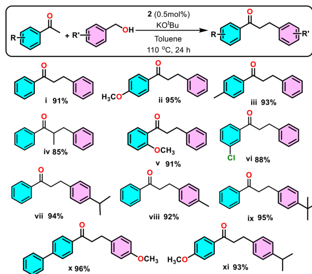
Scheme 2 Substrate scope for \alpha -alkylation reaction. General reaction conditions: acetophenone (0.50 mmol), benzyl alcohol (0.55 mmol), \text{KO}^t\text{Bu} (0.75 mmol), toluene 2 mL, 110 °C, and catalyst 2 (0.5 mol%). All are isolated yields.
