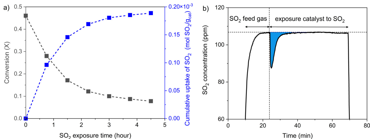
Fig. 1 a) Measured conversion and accumulated \text{SO}_2 uptake in six consecutive \text{SO}_2 exposure cycles at 200 °C after formation of the [(\text{NH}_3)_4\text{Cu}_2^{\text{II}}\text{O}_2]^{2+} complex. b) Measured \text{SO}_2 concentration during exposure to \text{SO}_2 . The blue area represents the uptake of \text{SO}_2 . Catalyst 3.2 wt% Cu-CHA, Si/Al ratio 6.7.
