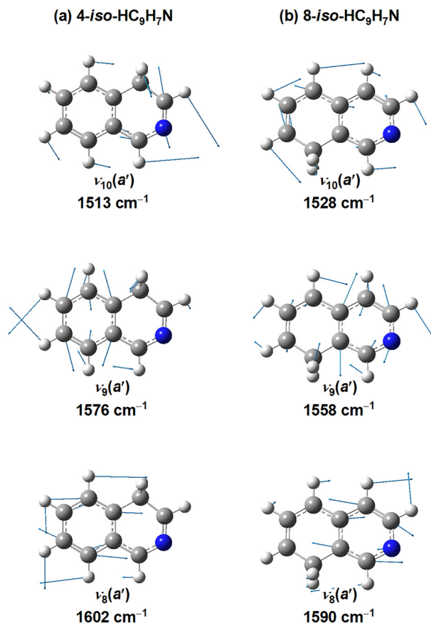
Fig. 5 Displacement vectors induced by the three a' C–C stretching modes of 4-iso-HC 9 H 7 N (a) and 8-iso-HC 9 H 7 N (b) in their electronic ground states calculated at the uB3PW91/6-311++G(2d,2p) level.
